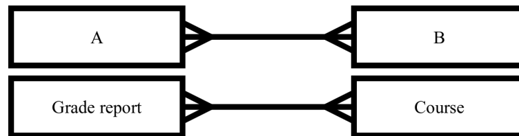
Figure 5: Many-to-many relationship.
